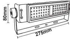
Dimension ( mm )
